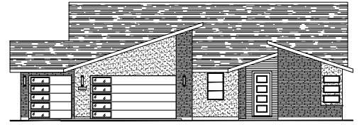
MODERN ELEVATION
